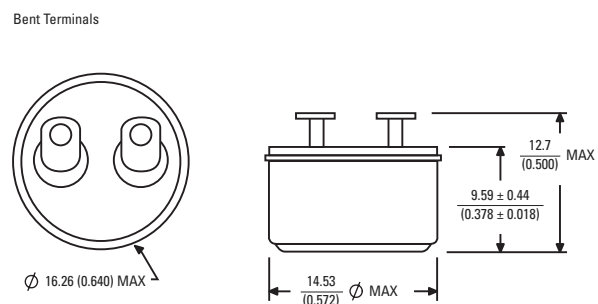
Bent Terminals
